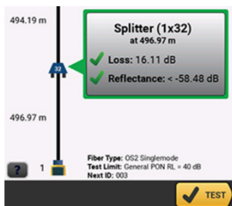
Splitter as seen on an EventMap
